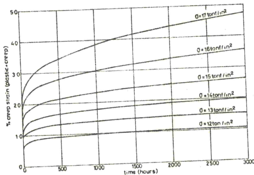
FIG. 7 EXPERIMENTAL TENSION CREEP CURVES FOR 0.18 PERCENT CARBON STEEL AT 400°C
